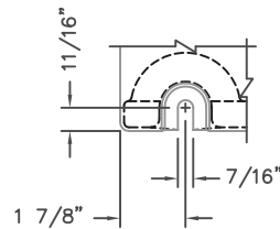
BOLT SLOT DETAIL
