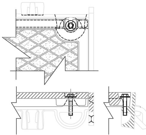
FRAME & GRATE SHOWING DEBRIS CHUTE
