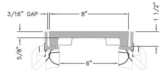
R-4999-AX TYPICAL SECTION TYPE "D" LID w/ TYPE "B" FRAME
